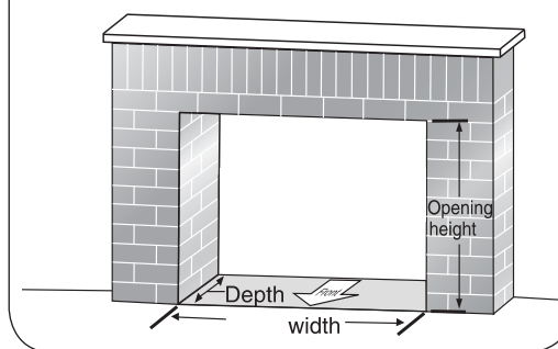
Fig. 5-1 Fireplace dimensions
