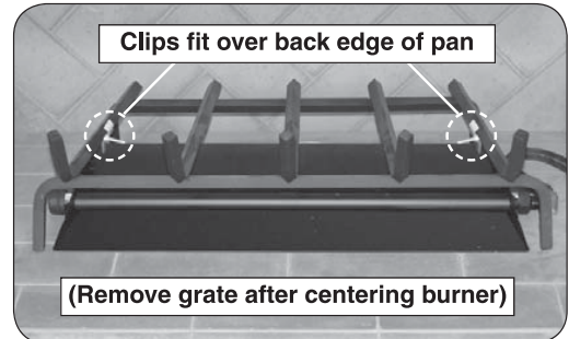
Fig. 10-2 Position grate
