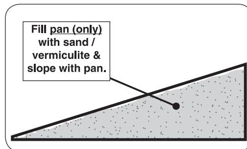
Fig. 11-2 Sand/vermiculite detail
