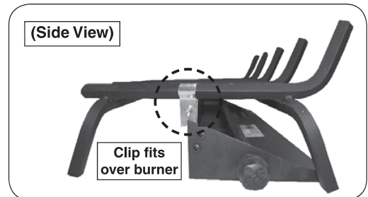
Fig. 10-3 Grate placement detail
