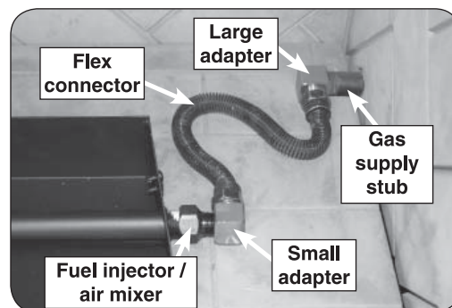
Fig. 9-1 Connect gas supply
