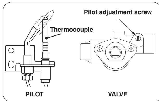
Fig. 39-1 Pilot adjustment detail
