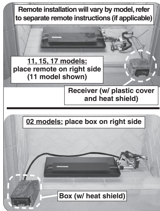
Fig. 18-1 Install remote receiver and heat shield (as applicable)
