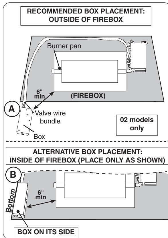
Fig. 17-3 Box placement (if applicable)
