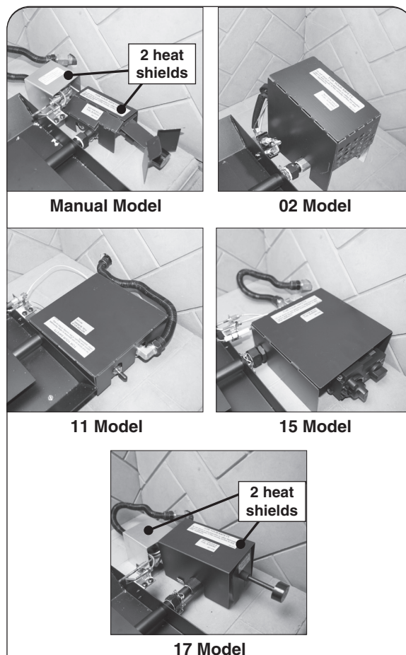
Fig. 18-1 Install remote receiver and heat shield (as applicable)
