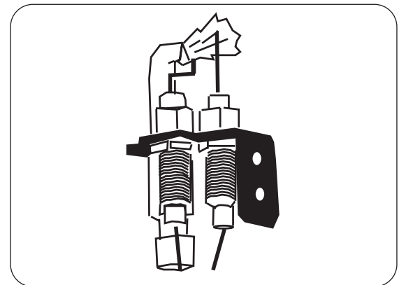
Fig. 29-2 Proper pilot flame
