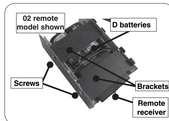
Fig. 21-3 Receiver/switch box batteries
