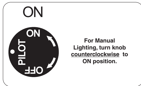
Fig. 37-3 Control knob detail (ON)
