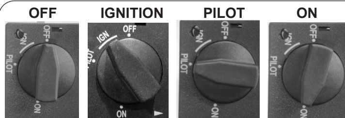
Ignition control knob - positions Fig. 33-1
