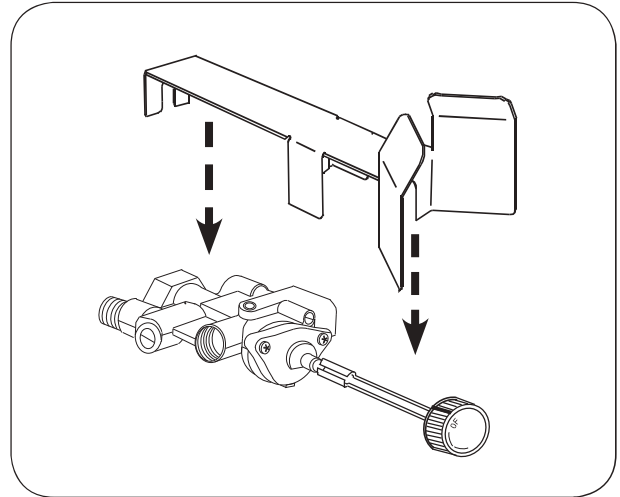
Fig. 8-1 Place heat shield
