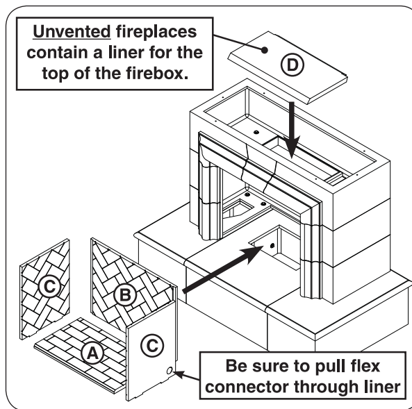
Fig. 19-1 Install firebox liners
