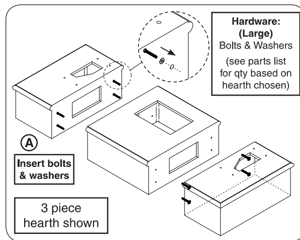
Fig. 16-1 Assemble hearth
