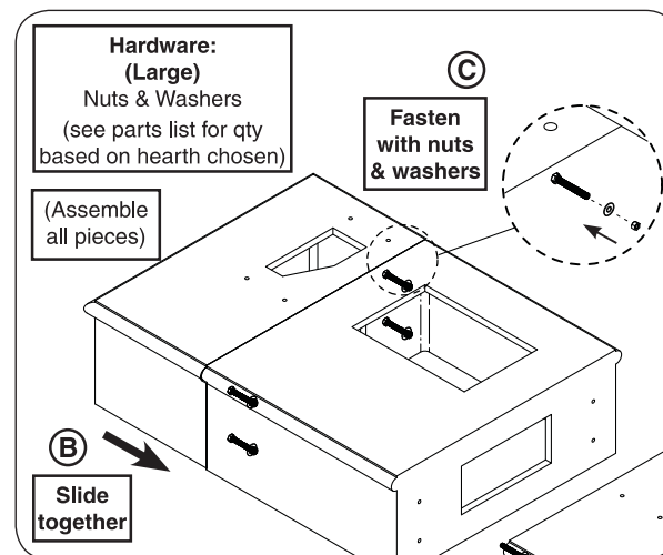
Fig. 16-2 Assemble hearth - slide together & fasten
