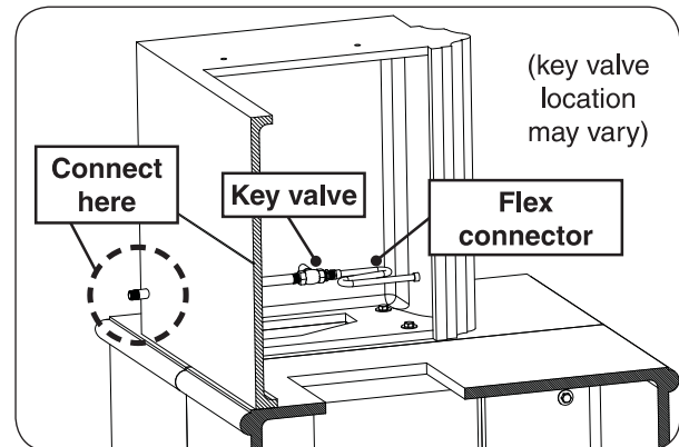
Fig. 17-2 Route gas supply (rear install)
