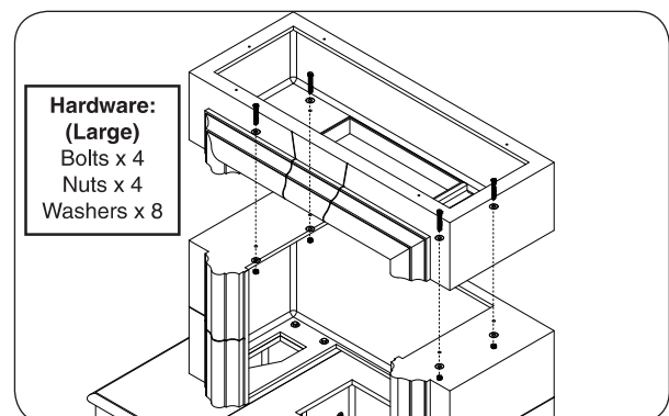
Fig. 17-4 Assemble middle body
