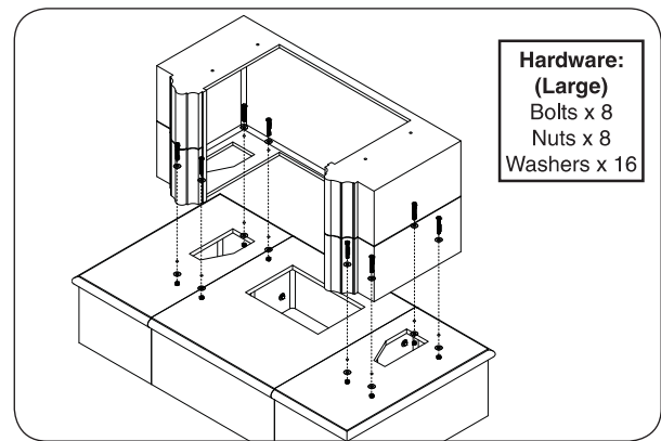
Fig. 17-1 Assemble base body
