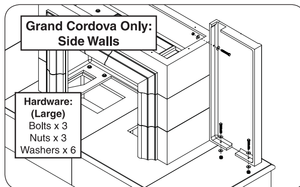
Fig. 18-2 Assemble rear side-wall (skip if n/a)
