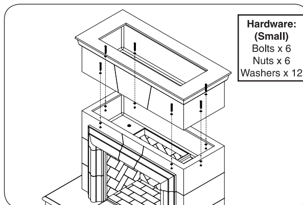
Fig. 19-2 Assemble top body
