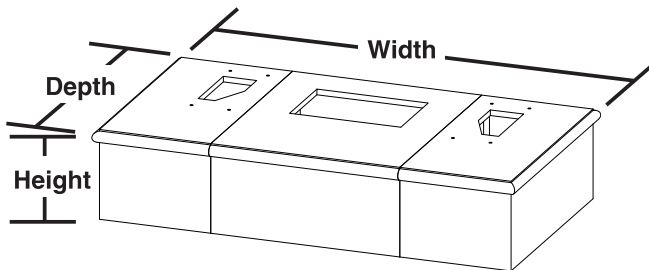
16" Rectangle Bullnose Hearth Shown
