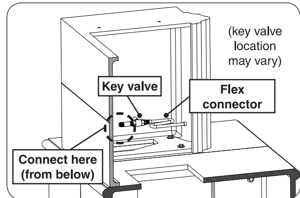
Fig. 17-3 Route gas supply (underneath install)
