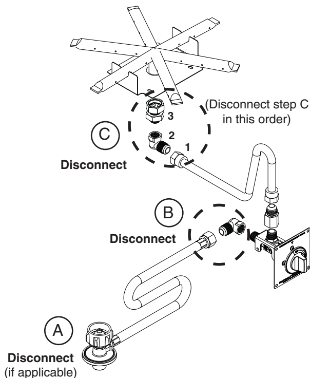
Fig. 3-1 Original configuration (L.P. gas)
