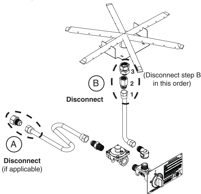
Fig. 5-1 Original configuration (L.P. gas)
