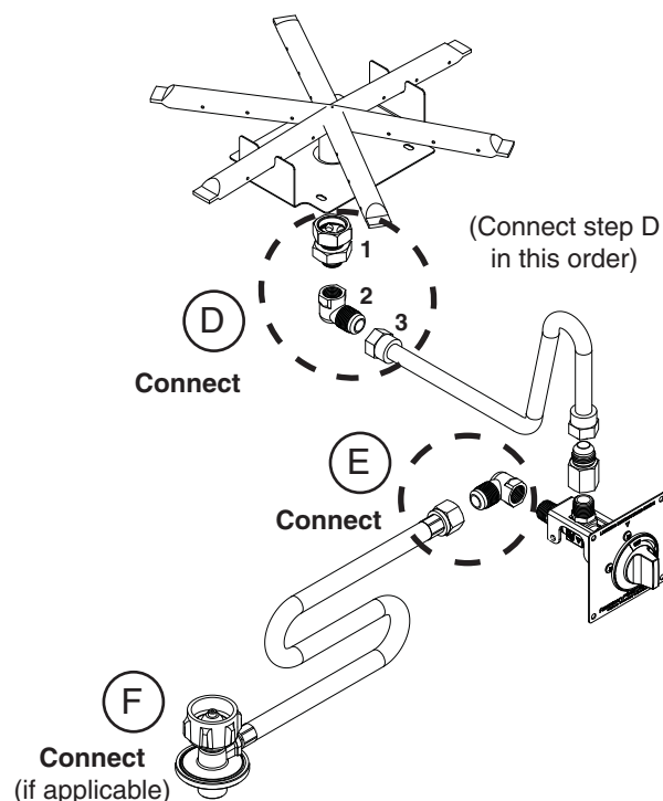
Fig. 4-2 New configuration (L.P. gas)
