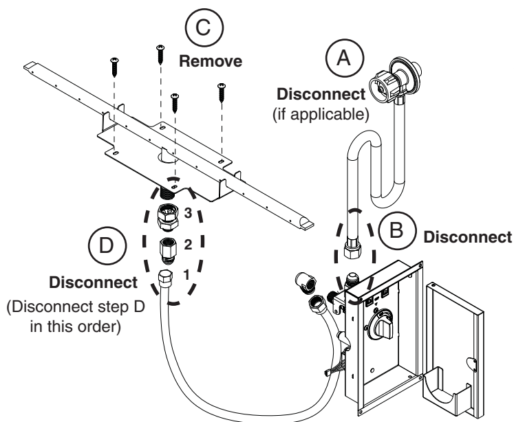
Fig. 9-1 Original configuration (L.P. gas)
