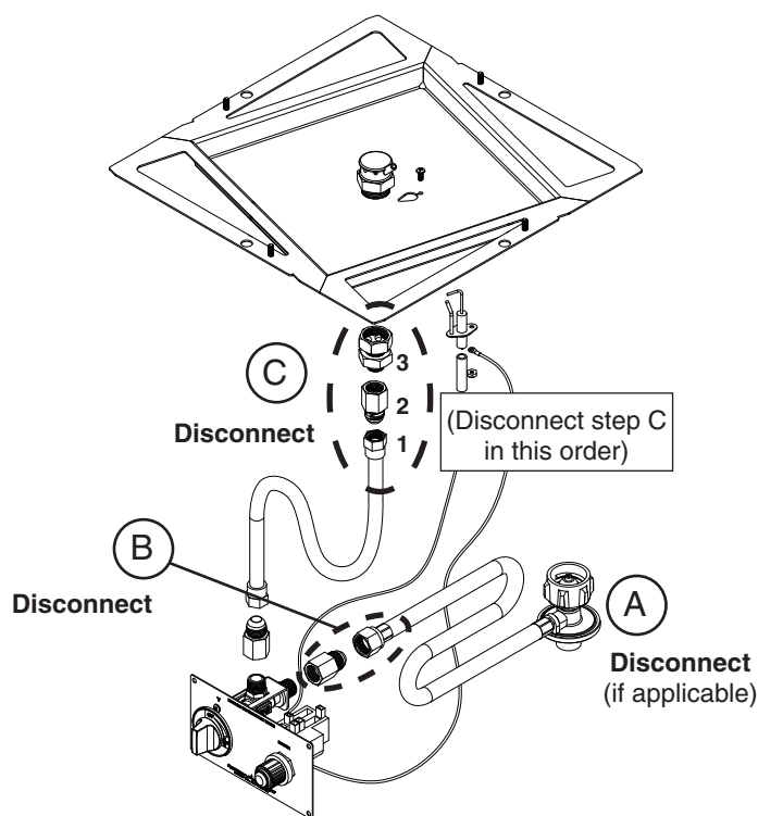
Fig. 7-1 Original configuration (L.P. gas)
