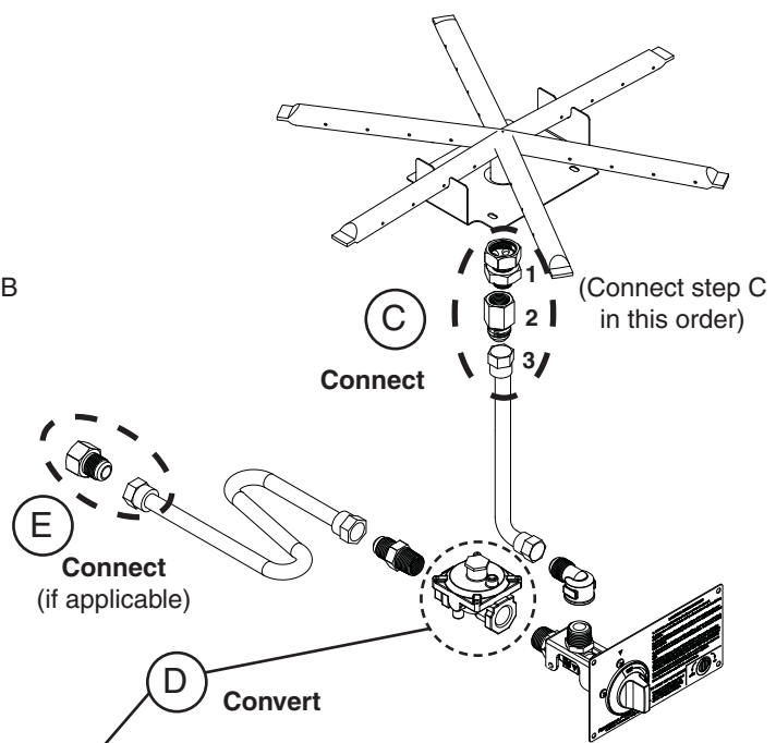
Fig. 6-2 New configuration (L.P. gas)
