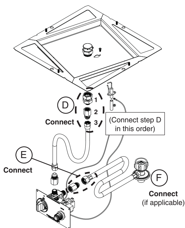
Fig. 8-2 New configuration (L.P. gas)
