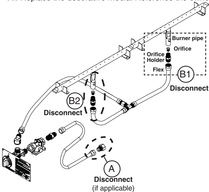
Fig. 13-1 Original configuration (L.P. gas)
