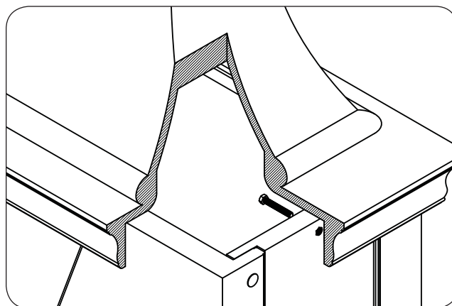
Fig. 21-3 Bolt detail
