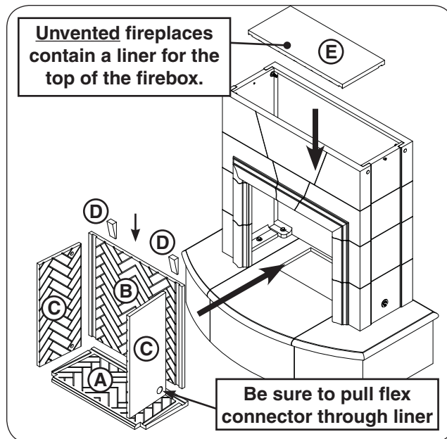
Fig. 21-1 Install firebox liners
