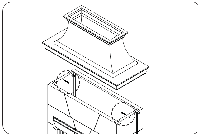
Fig. 21-2 Assemble chimney
