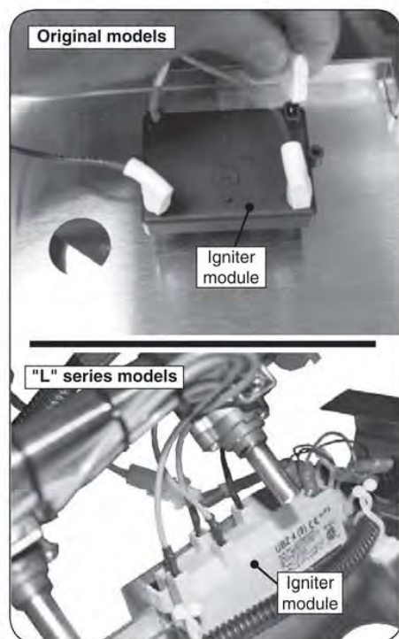
Fig. 2-2 Remove old igniter wire
