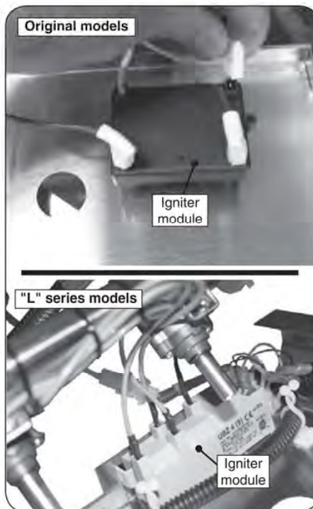
Fig. 4-2 Connect wire to the igniter module
