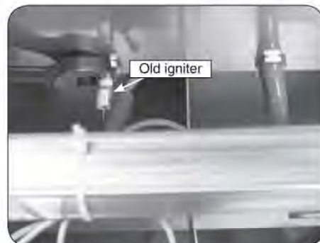
Fig. 2-1 Remove old igniter electrode
