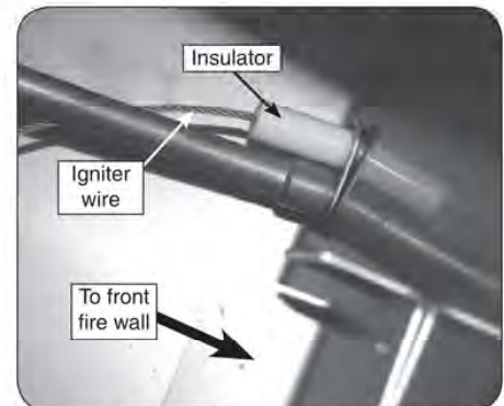
Fig. 3-2 Screw in the new wire insulator
