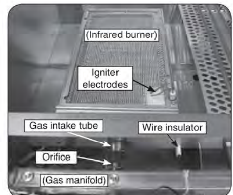
Fig. 3-4 Infrared burner installed
