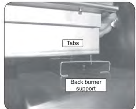
Fig. 3-3 Setting tabs into support
