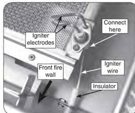
Fig. 4-1 Connect bare wire to electrode assy.
