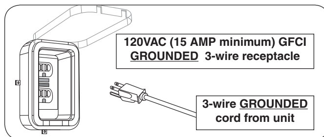
Fig. 18-4 Electrical setup detail
