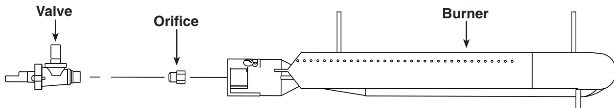
Fig. 27-1 - Main burner orifice diagram
