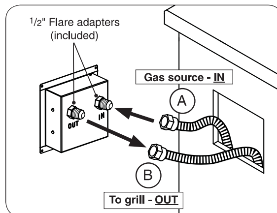
Fig. 1-2 Install timer box
