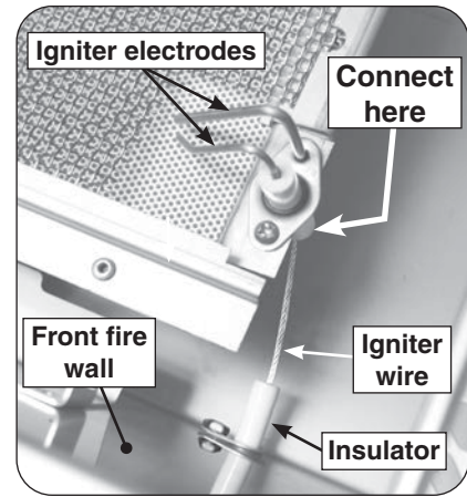
Fig. 4-1 Connect wire to electrode assy.
