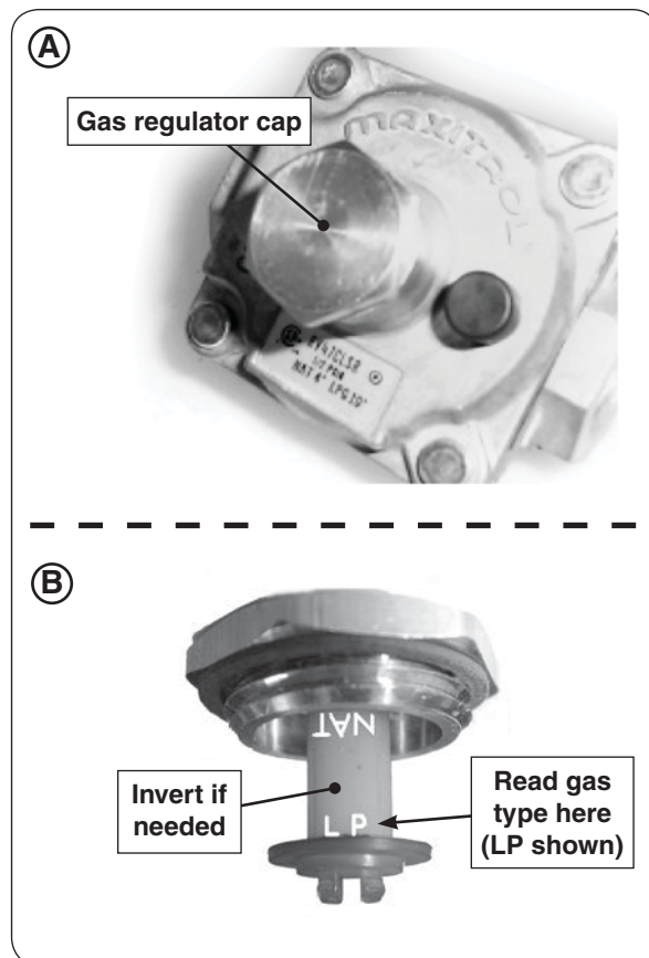
Fig. 30-1 Convert regulator
