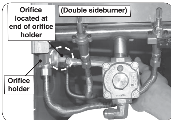
Fig. 31-4 Double sideburner orifice locations
