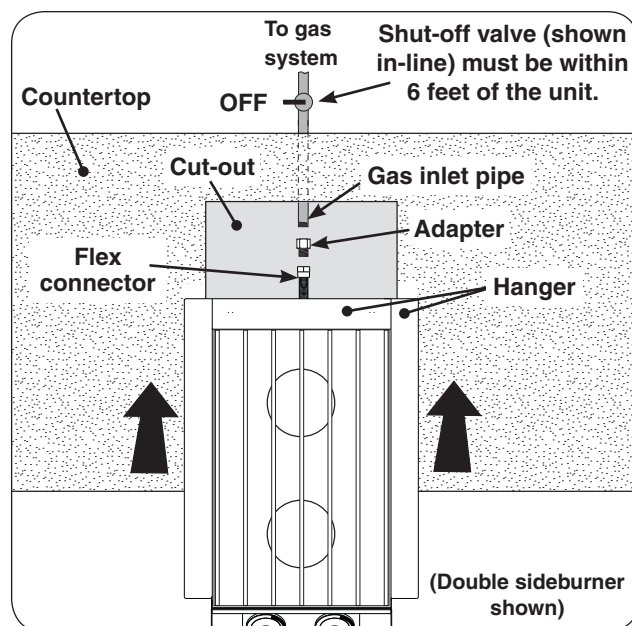
Fig. 19-4 Household propane & natural gas diagram
