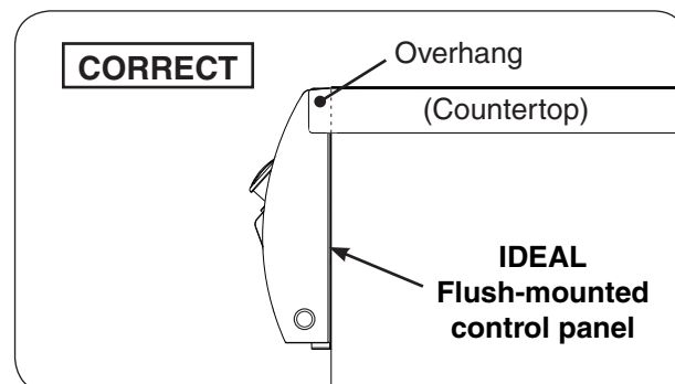
Fig. 19-2 Countertop overhang - correct cutout
