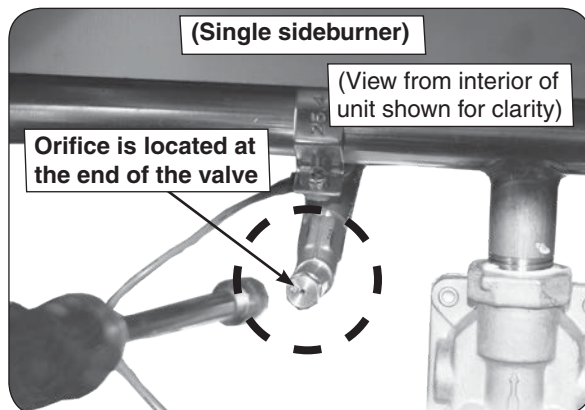
Fig. 31-3 Single sideburner orifice location
