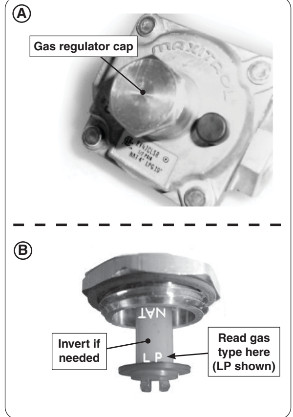
Fig. 32-1 Convert regulator
