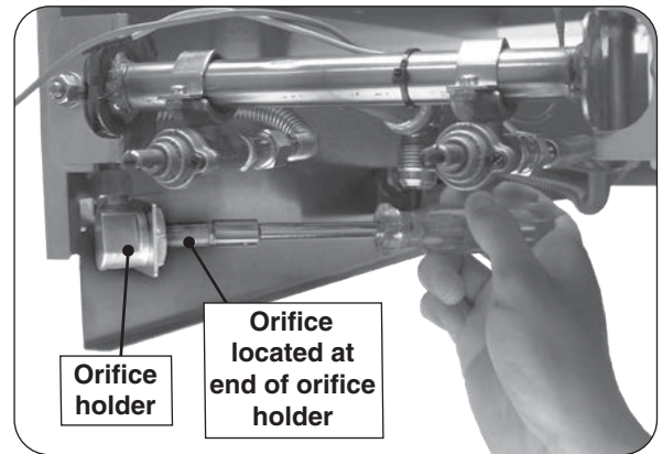
Fig. 33-1 Orifice location
