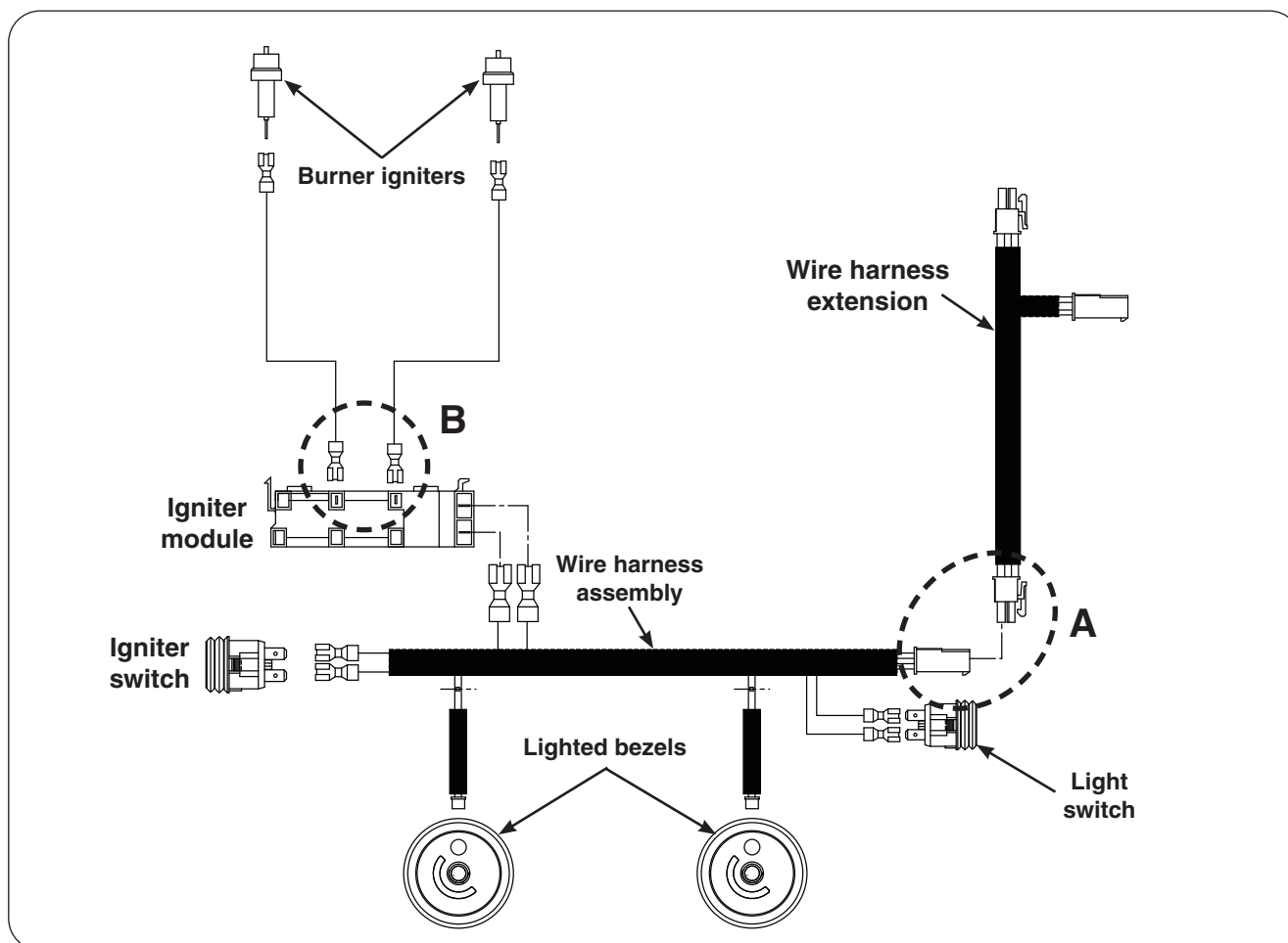
Fig. 30-1 - Wire diagram
